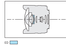
LUMIX G FISHEYE 8mm / F3.5 (H-F008) MULTI COATING
