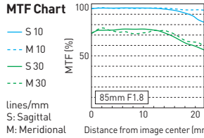
For lenses that are capable of compensating distortion, the horizontal axis of the MTF shows the distance from the center of the corrected image.
