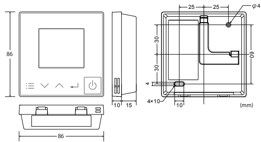
SIMPLIFIED WIRED REMOTE CONTROLLER (CZ-RTC6 / CZ-RTC6BL)
